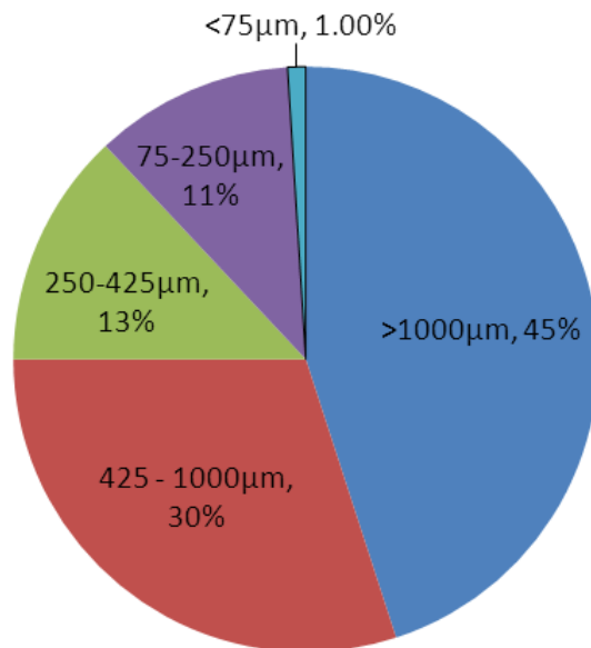
Figure 5 Total percentage of particle mass retained by the 1000 \mu m, 425 \mu m, 250 \mu m, 75 \mu m and pan (<75 \mu m) sieve cloths
